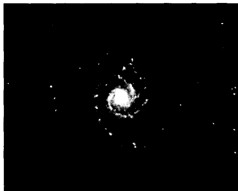
NGC 628 M74 Type Sc
