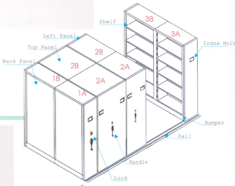
MCF 1 W2075 X D3100 X H2045 mm 81.69 X 122.0 X 80.51 inches
