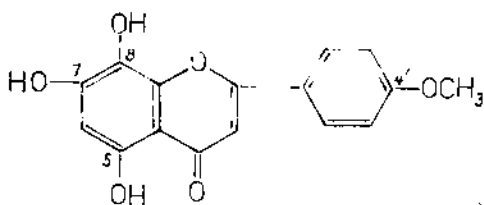
Chất (II) 5,7,8 - trihydroxy - 4' - methoxyflavon C_{16}H_{12}O_6
