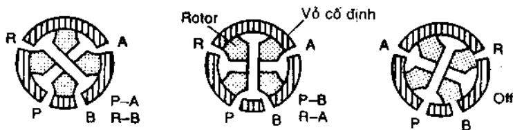
(a) Valve 4/3
