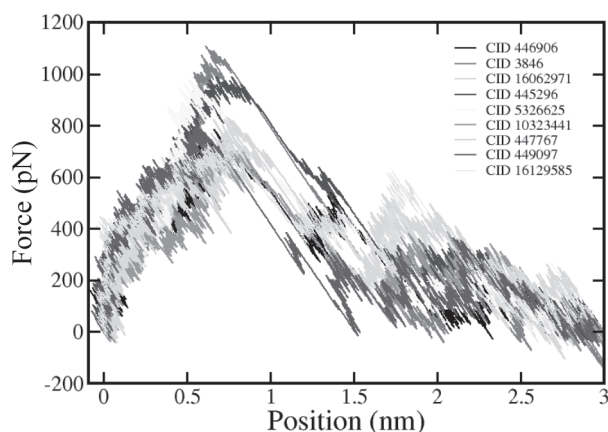
Figure 8. Force-position profiles obtained by the SMD method
