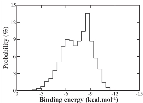
Figure 5. Distributions of binding energies of 5732 ligands to receptor
