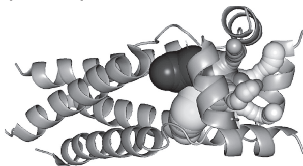
Figure 3. Some pulling directions of CID 5326625 by Caver 3.0
