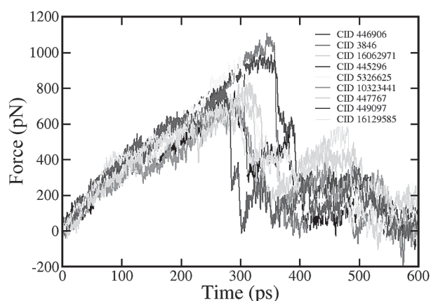
Figure 9. Force-time profiles obtained by the SMD method
