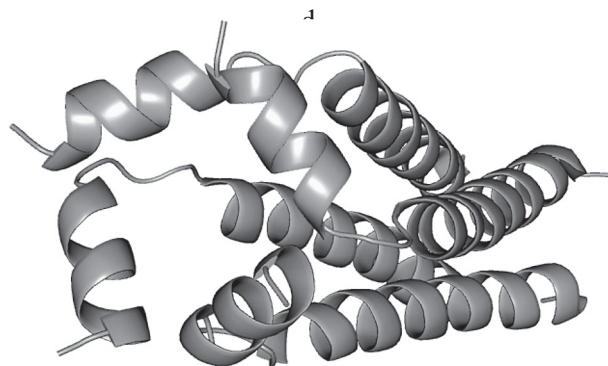
Figure 2. The structure of channel M2 from influenza A (2RLF) virus H5N1
