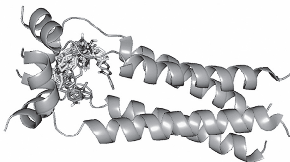
Figure 4. Locations of these compounds in proton channel M2 from influenza A
