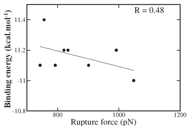
Figure 7. The Correlation coefficient between rupture force and binding energy
