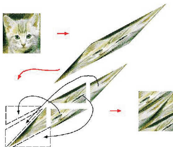
Figure 1. The Arnold's cat map
