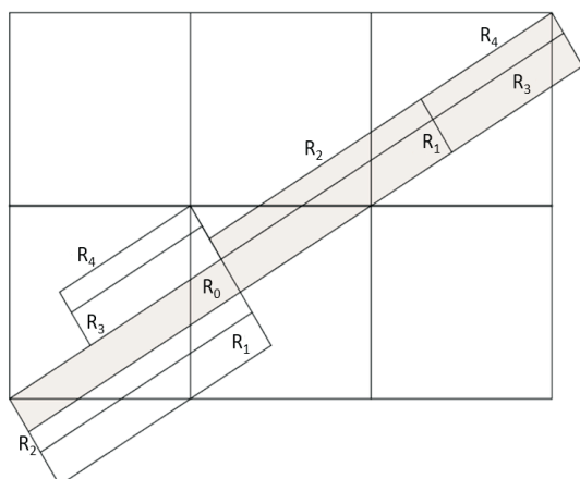
Figure 2. A Markov partition of T_A .
