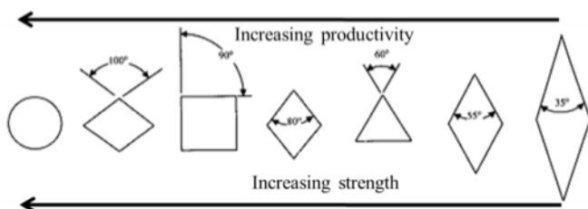
Fig. 3. Insert shape with respect to strength and productivity
