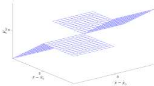
Figure 6. Damping force F_{SA} with respect to (x - x_0) and (\dot{x} - \dot{x}_0) in case of the continuous balance control
